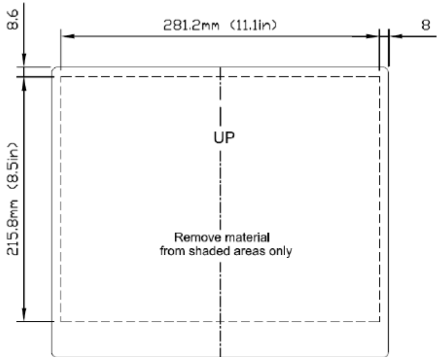
Back View
